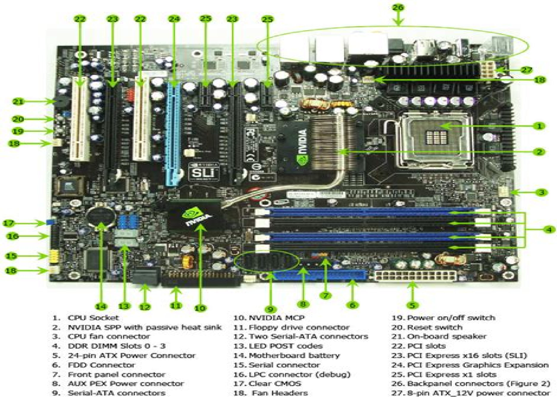
Figure 1. EVGA nForce 680i SLI Motherboard Layout
